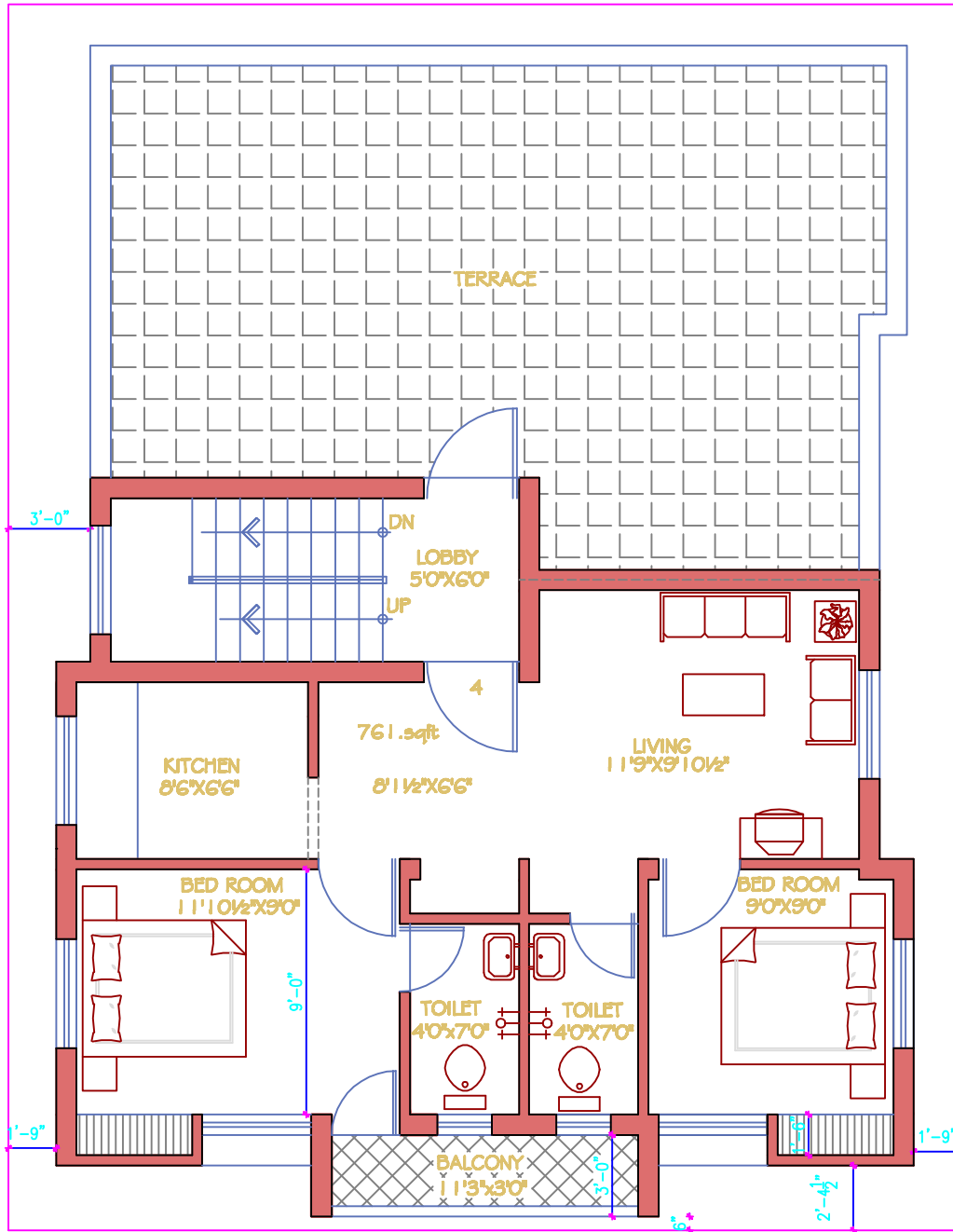
SITE CUM SECOND FLOOR PLAN
